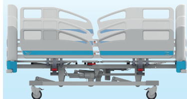
43-78,5cm Height Movement
